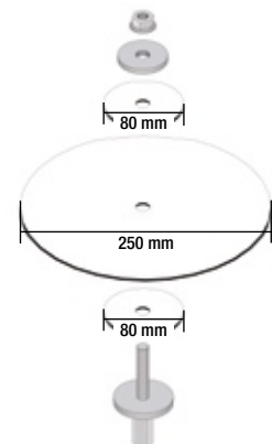
MAPEPLAN® T ANCHORING INOX BF 16 mm
