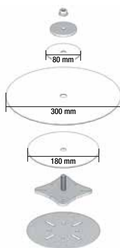
MAPEPLAN® ANCHORING INOX LIGHT
